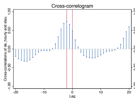
FIGURE 5.— A cross correlogram between the hourly number of ADAC traffic jam reports and the hourly Google search intensity for stau establishes that Google search has a two hour advance on road conditions.
